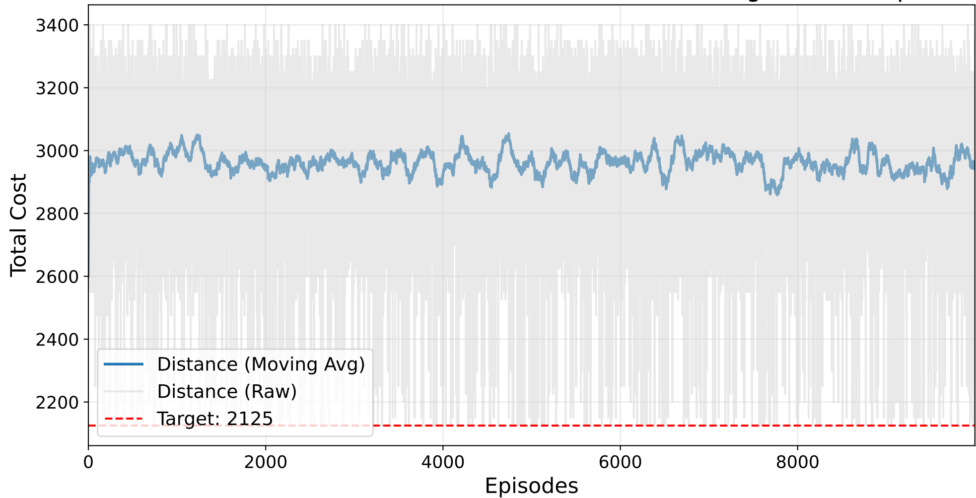
Final HYPERBAND TPE Masked AutoRL-SOP Training - ESC07.sop
